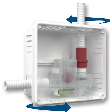
SCARICO REVERSIBILE DESCARGA REVERSIBLE REVERSIBLE OUTLET
